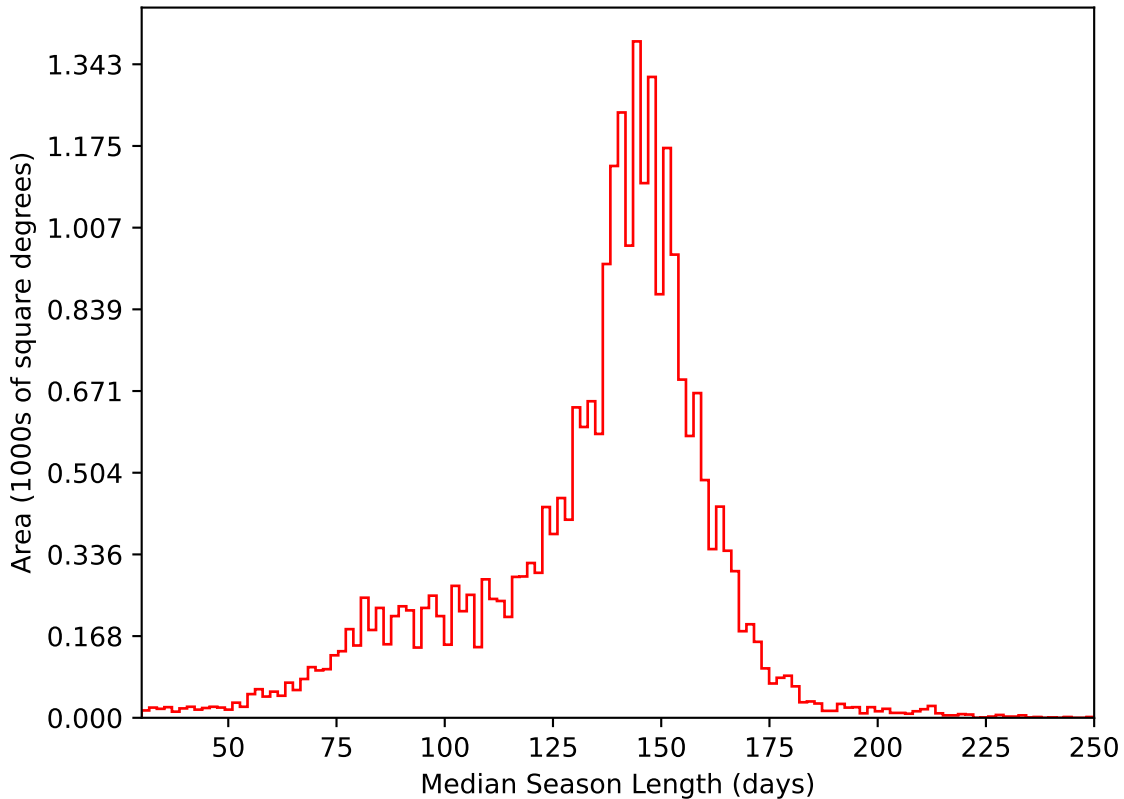
ddf_loaded_half_fl4_v3.4_10yrs All sky i band: Median Season Length
