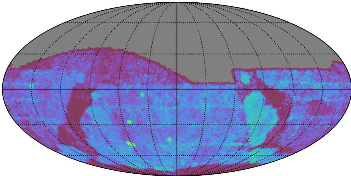
ddf_loaded_half_fl4_v3.4_10yrs All sky g band: Median Season Length
