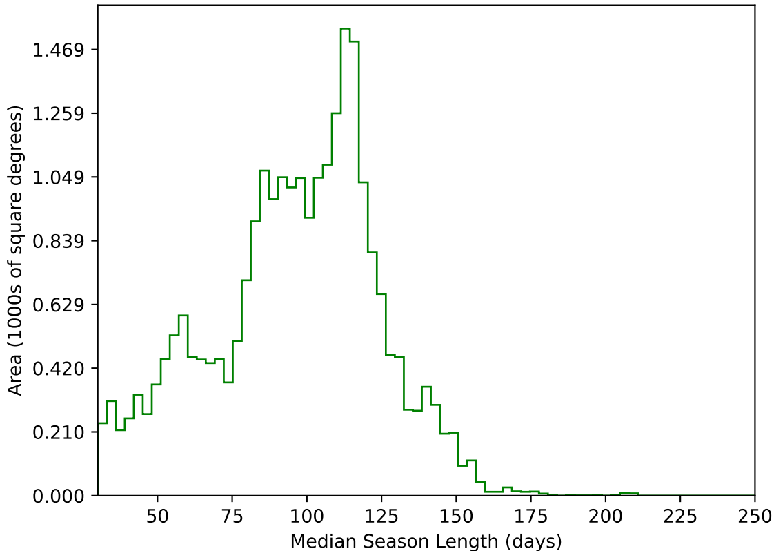
ddf_loaded_half_fl4_v3.4_10yrs All sky g band: Median Season Length
