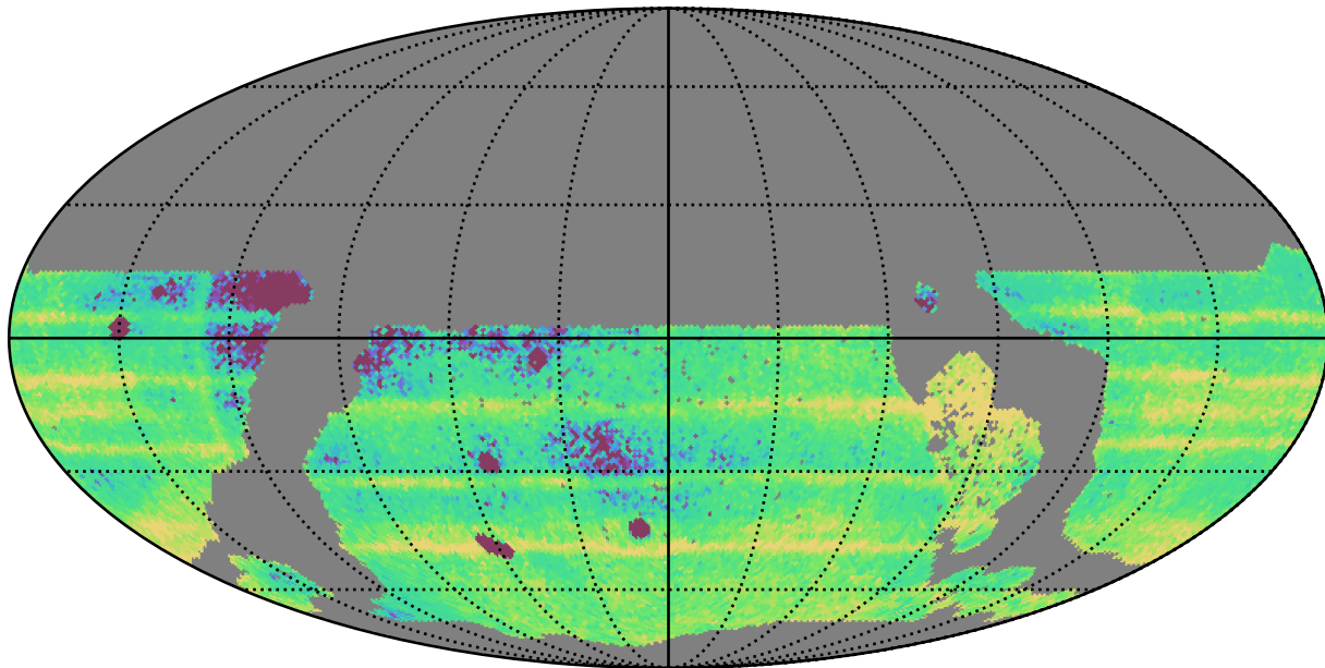
ddf_loaded_half_fl4_v3.4_10yrs WFD: Median Intra-Night Gap
