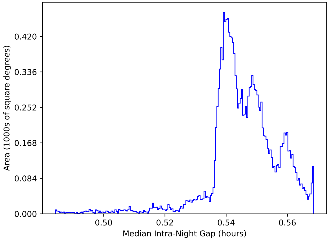
ddf_loaded_half_fl4_v3.4_10yrs WFD: Median Intra-Night Gap
