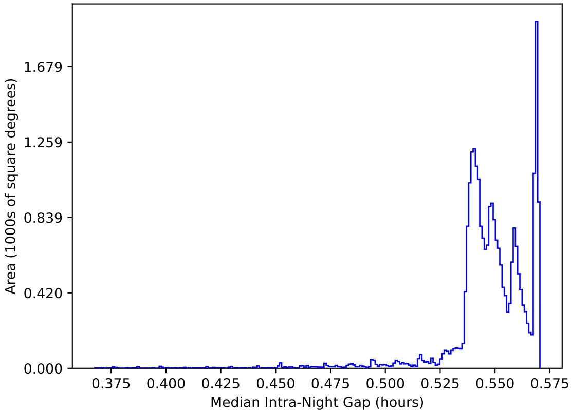
ddf_loaded_half_fl4_v3.4_10yrs All sky: Median Intra-Night Gap
