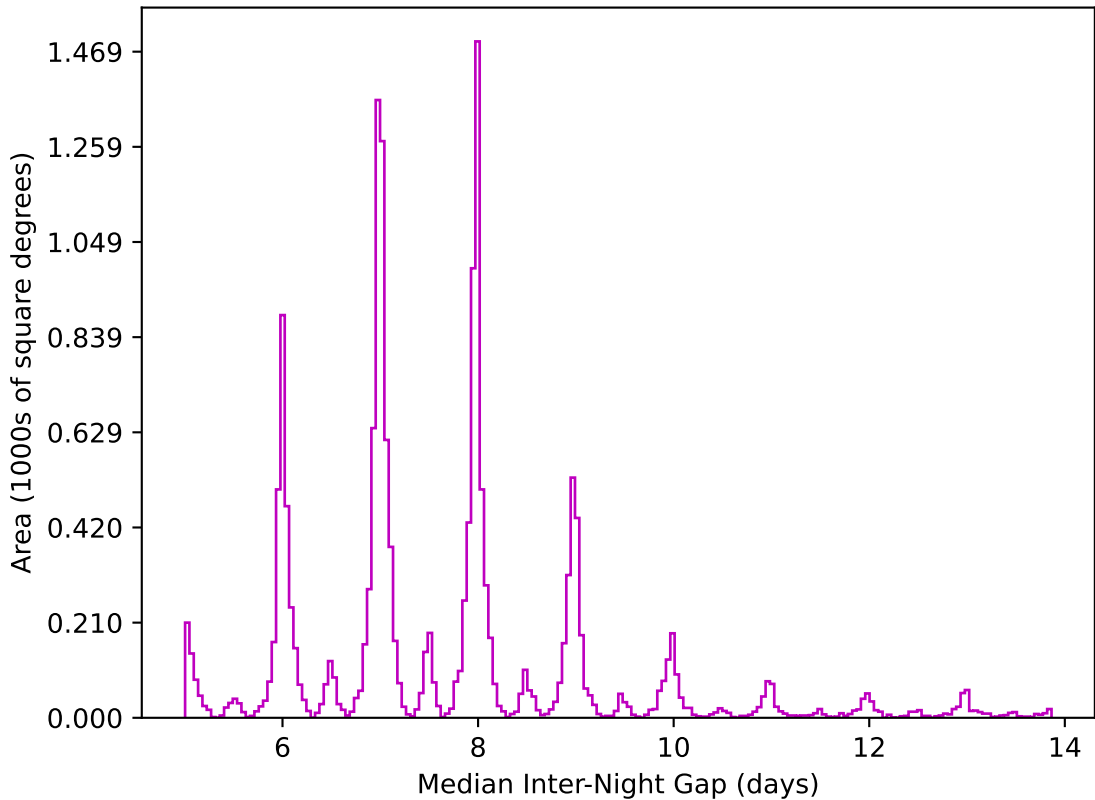
ddf_loaded_half_fl4_v3.4_10yrs WFD z band: Median Inter-Night Gap
