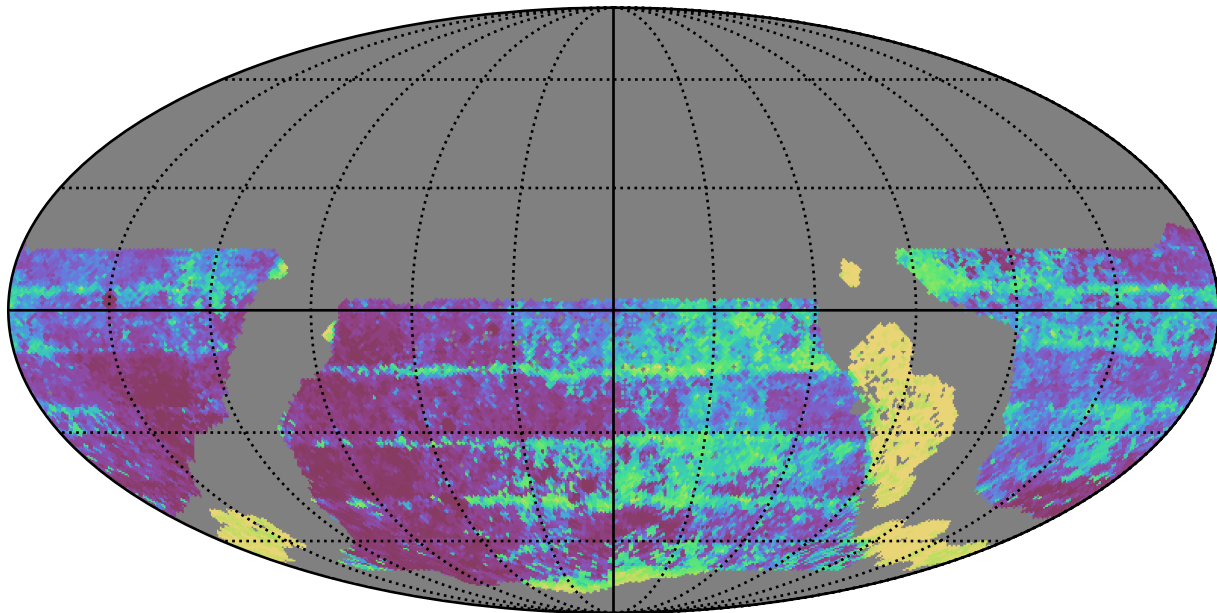
ddf_loaded_half_fl4_v3.4_10yrs WFD y band: Median Inter-Night Gap
