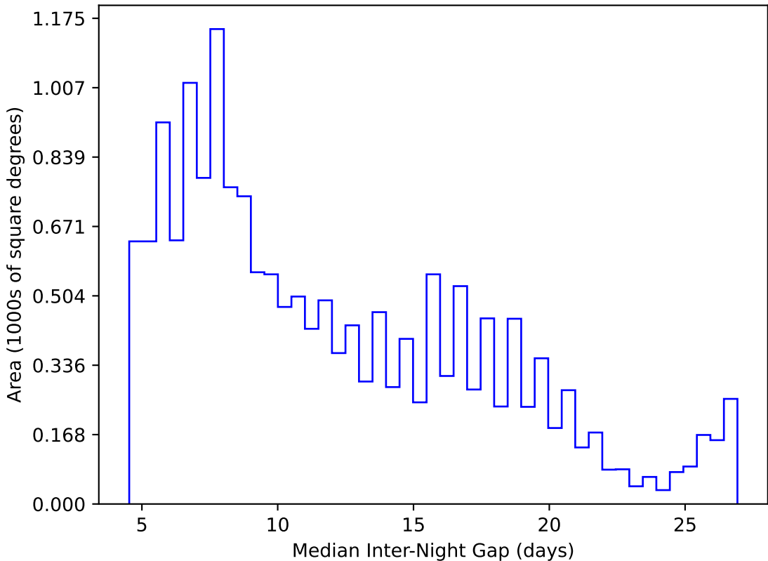
ddf_loaded_half_fl4_v3.4_10yrs WFD y band: Median Inter-Night Gap
