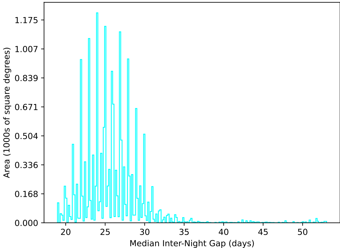
ddf_loaded_half_fl4_v3.4_10yrs WFD u band: Median Inter-Night Gap
