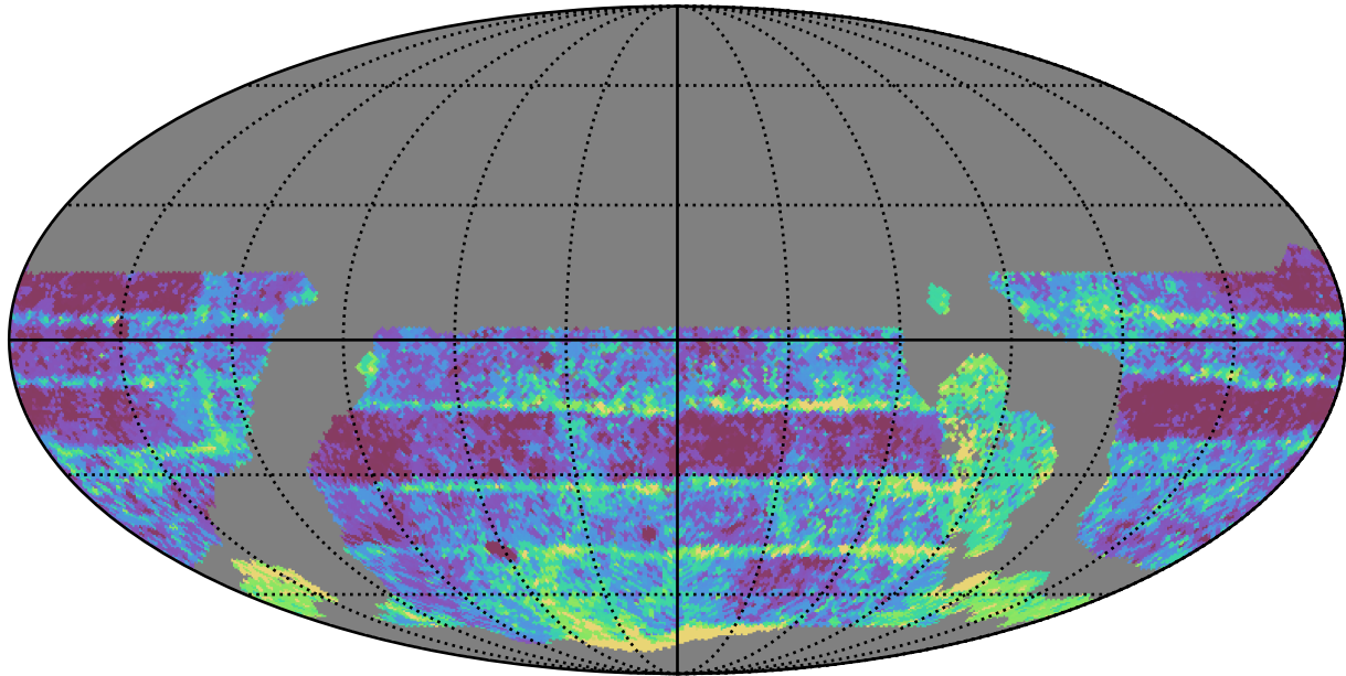
ddf_loaded_half_fl4_v3.4_10yrs WFD r band: Median Inter-Night Gap
