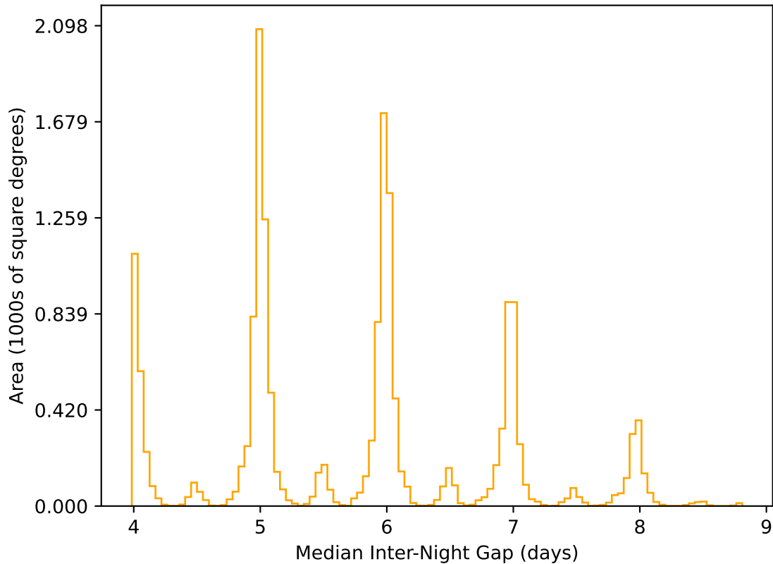
ddf_loaded_half_fl4_v3.4_10yrs WFD r band: Median Inter-Night Gap
