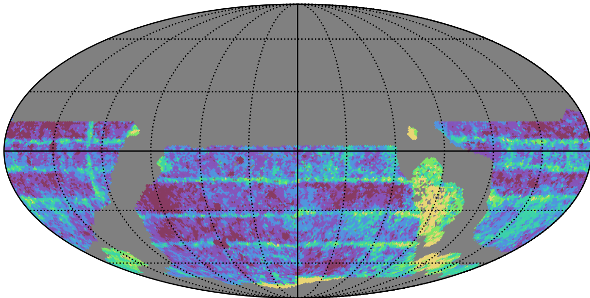
ddf_loaded_half_fl4_v3.4_10yrs WFD i band: Median Inter-Night Gap
