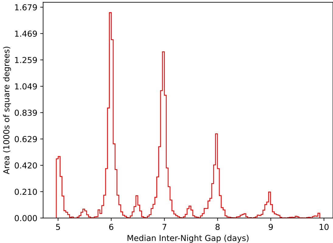
ddf_loaded_half_fl4_v3.4_10yrs WFD i band: Median Inter-Night Gap
