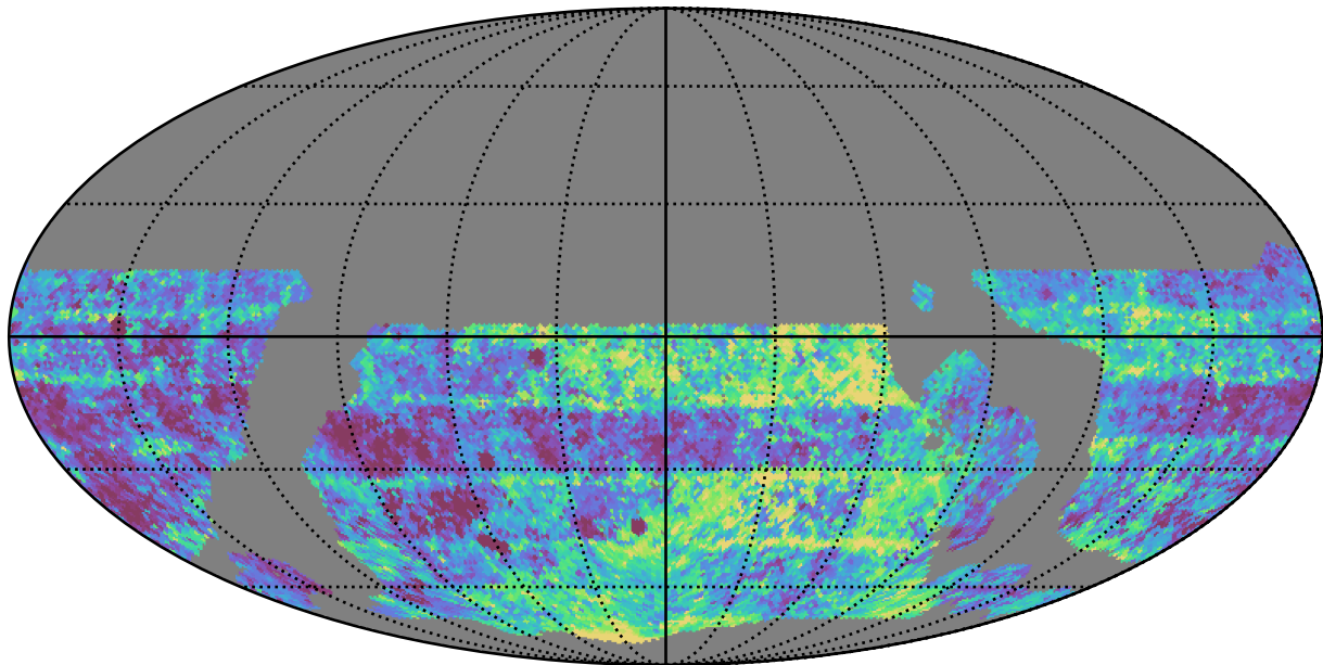
ddf_loaded_half_fl4_v3.4_10yrs WFD g band: Median Inter-Night Gap
