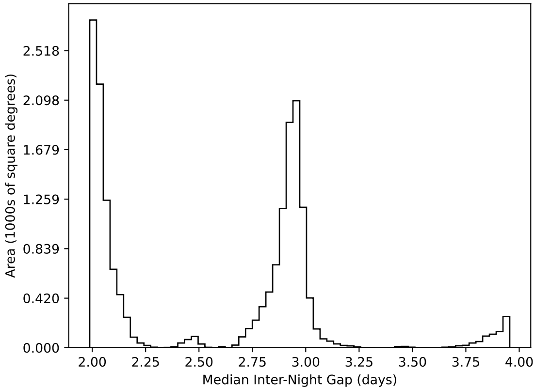
ddf_loaded_half_fl4_v3.4_10yrs WFD all bands: Median Inter-Night Gap
