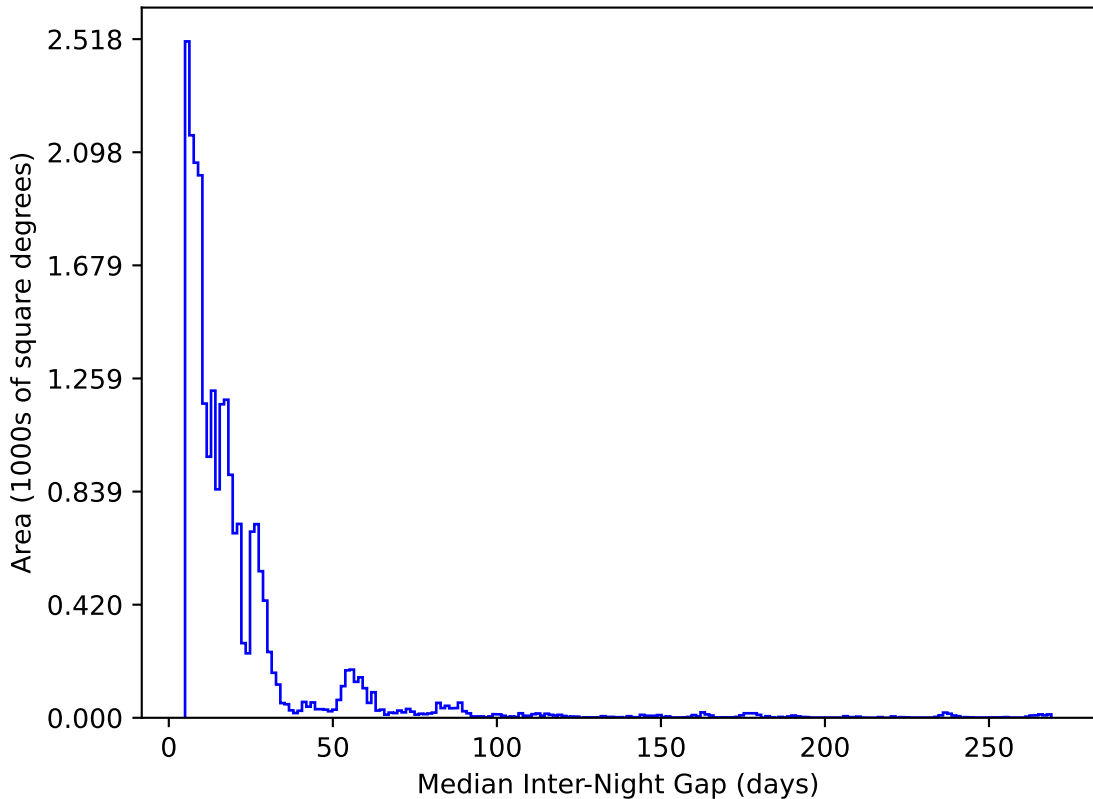
ddf_loaded_half_fl4_v3.4_10yrs All sky y band: Median Inter-Night Gap
