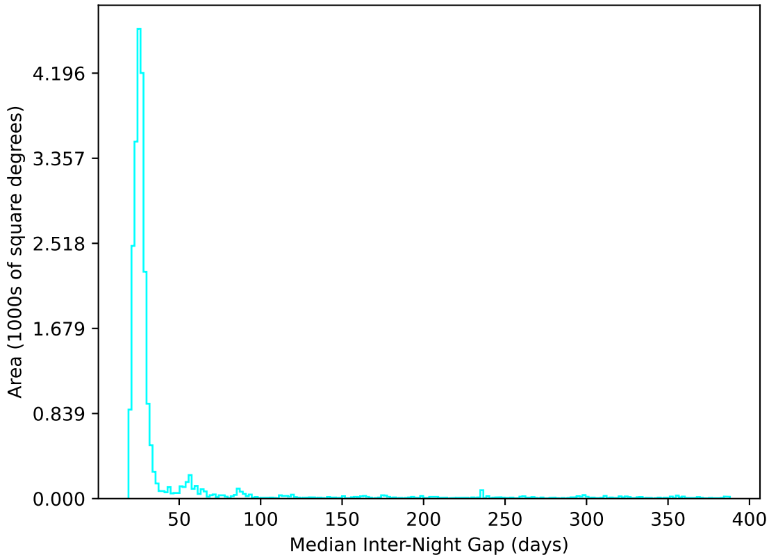
ddf_loaded_half_fl4_v3.4_10yrs All sky u band: Median Inter-Night Gap
