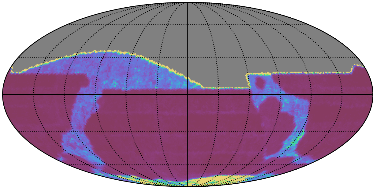
ddf_loaded_half_fl4_v3.4_10yrs All sky r band: Median Inter-Night Gap
