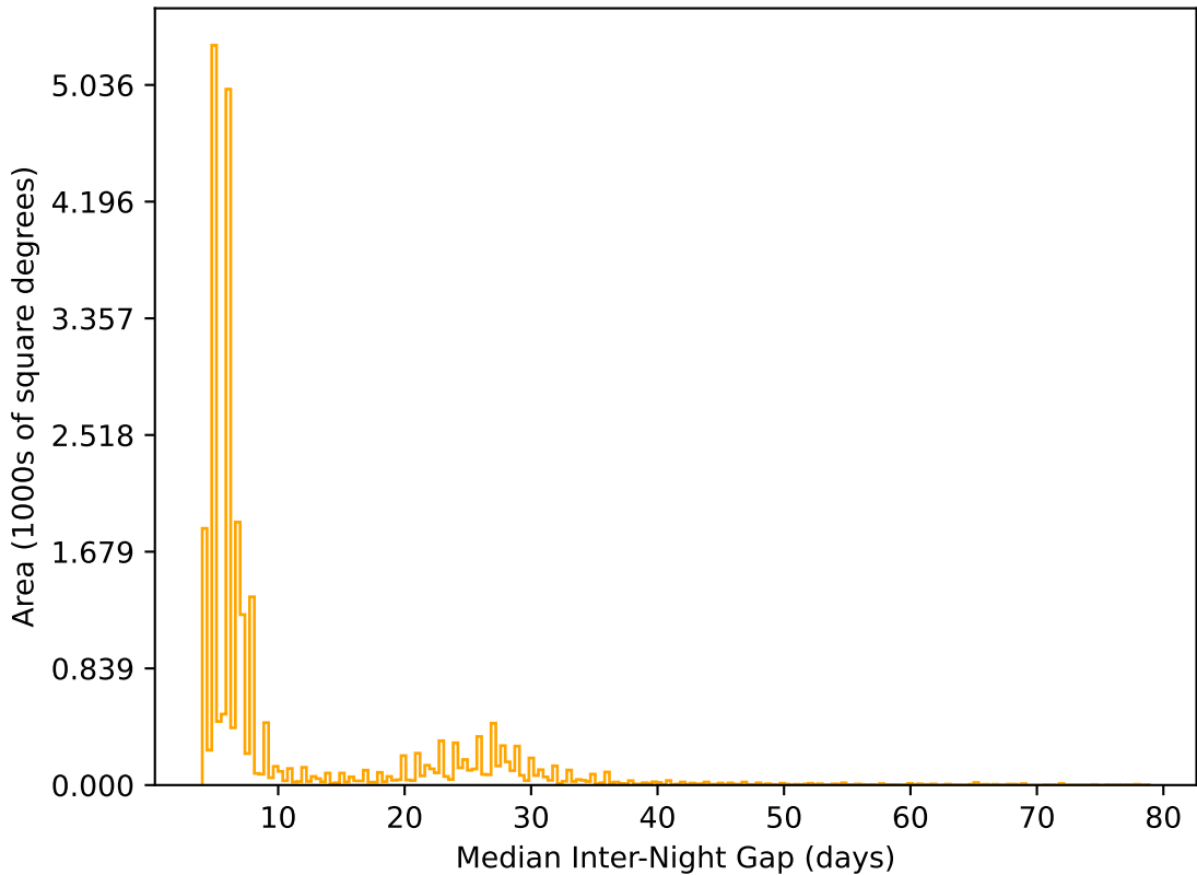
ddf_loaded_half_fl4_v3.4_10yrs All sky r band: Median Inter-Night Gap
