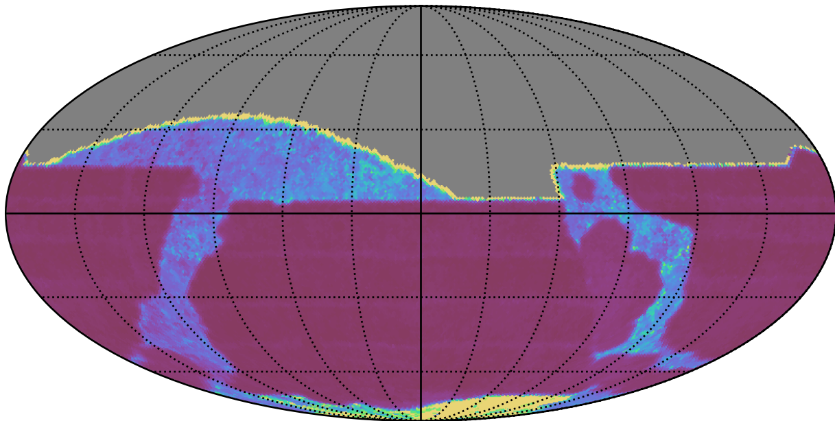
ddf_loaded_half_fl4_v3.4_10yrs All sky i band: Median Inter-Night Gap
