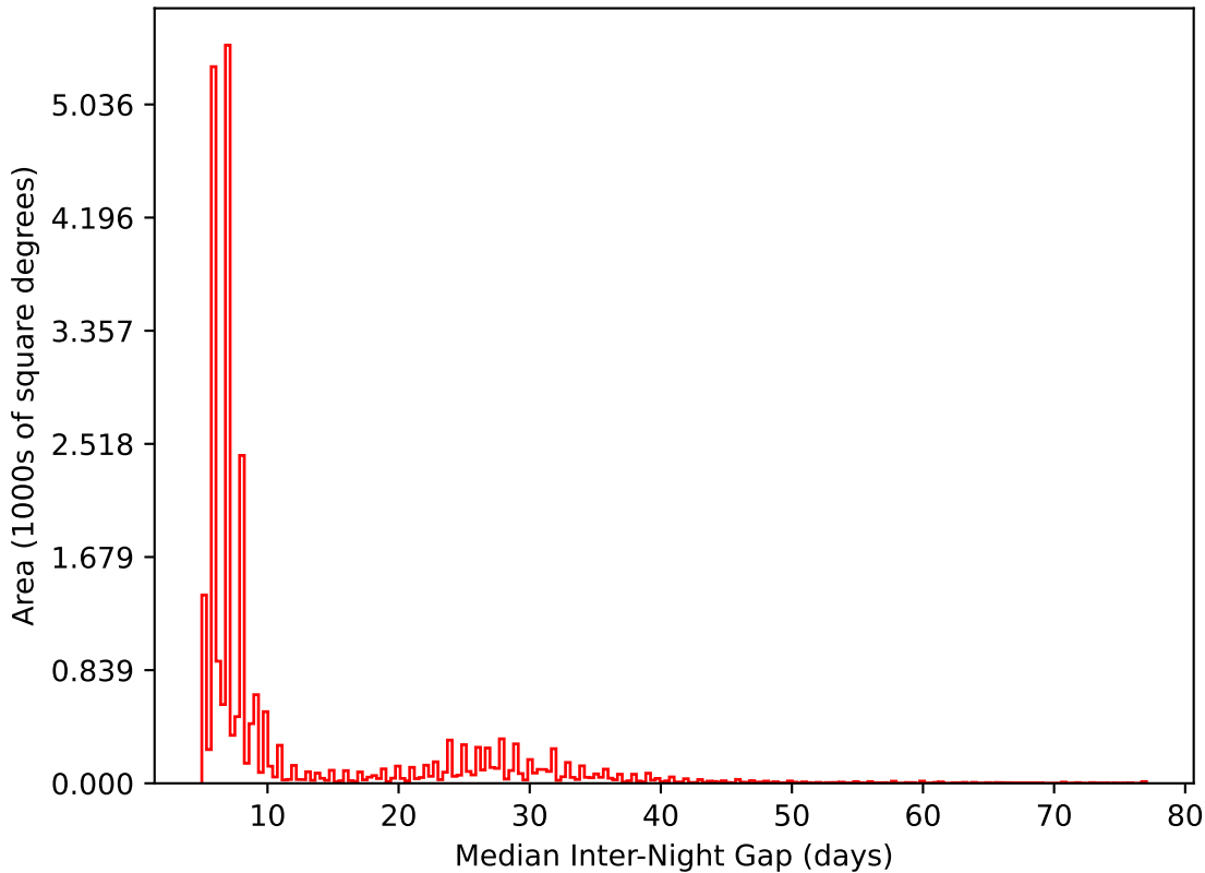
ddf_loaded_half_fl4_v3.4_10yrs All sky i band: Median Inter-Night Gap
