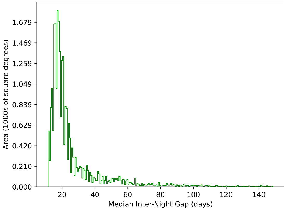
ddf_loaded_half_fl4_v3.4_10yrs All sky g band: Median Inter-Night Gap
