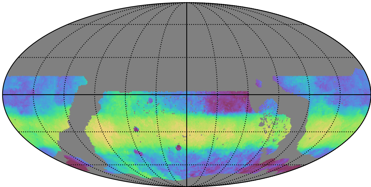
ddf_loaded_half_fl4_v3.4_10yrs WFD z band: Median HA
