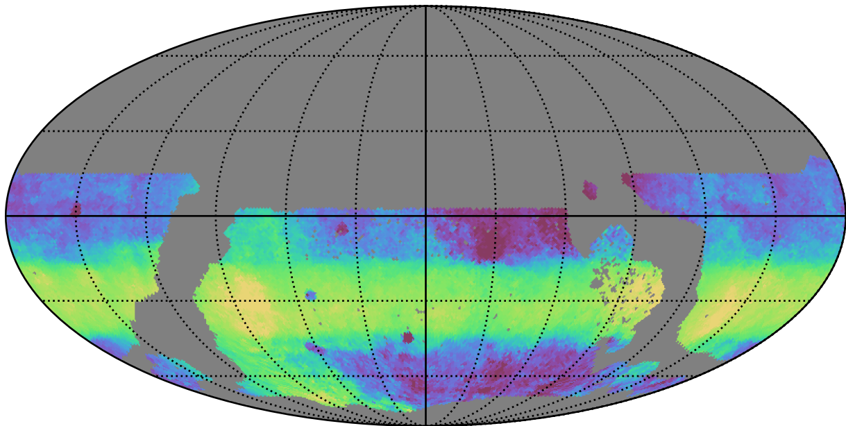
ddf_loaded_half_fl4_v3.4_10yrs WFD y band: Median HA
