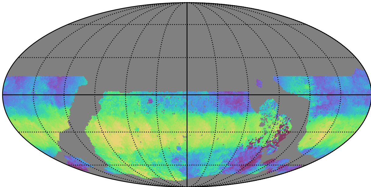
ddf_loaded_half_fl4_v3.4_10yrs WFD u band: Median HA
