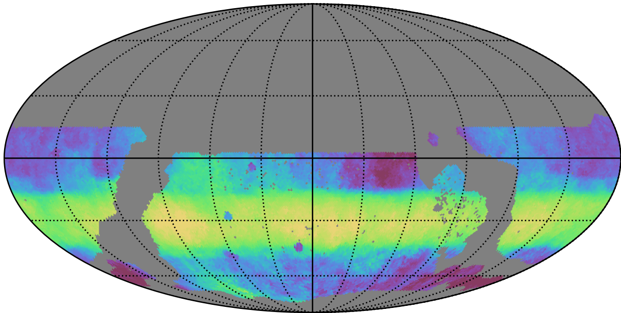
ddf_loaded_half_fl4_v3.4_10yrs WFD i band: Median HA
