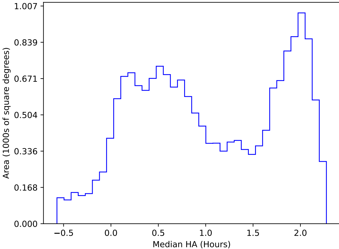
ddf_loaded_half_fl4_v3.4_10yrs WFD i band: Median HA
