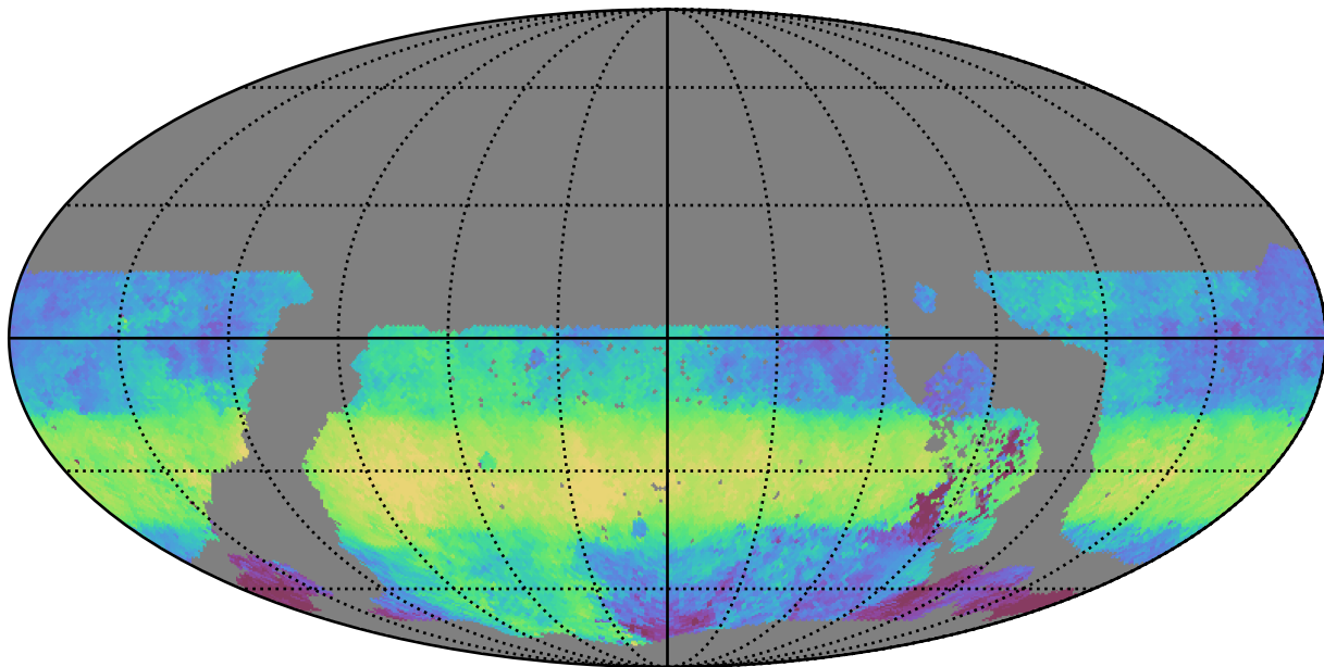
ddf_loaded_half_fl4_v3.4_10yrs WFD g band: Median HA
