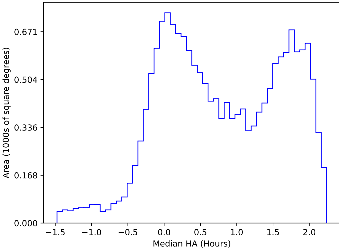
ddf_loaded_half_fl4_v3.4_10yrs WFD g band: Median HA
