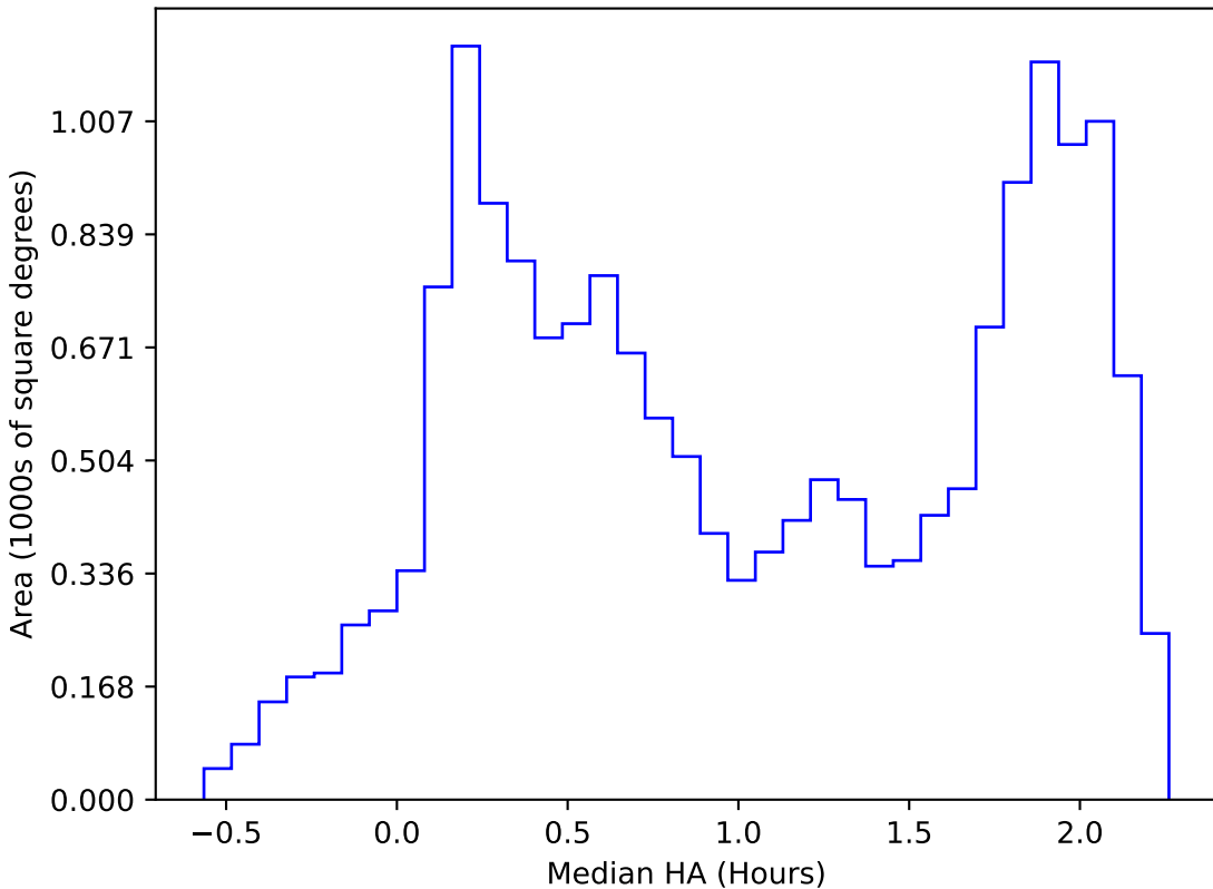
ddf_loaded_half_fl4_v3.4_10yrs WFD all bands: Median HA
