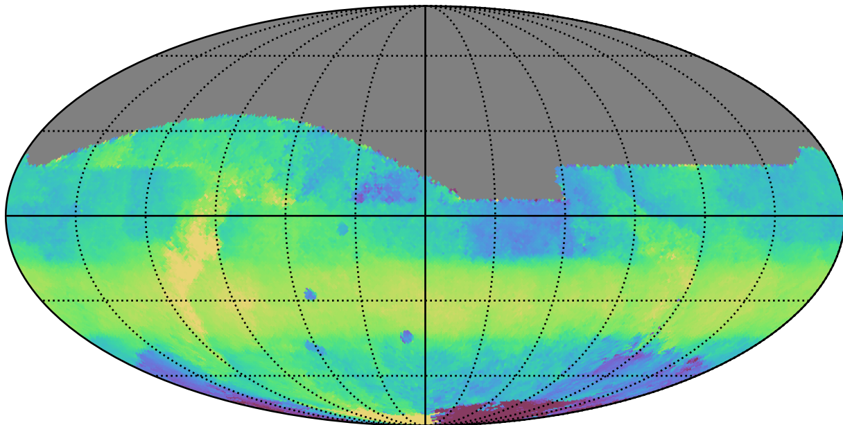
ddf_loaded_half_fl4_v3.4_10yrs All sky z band: Median HA
