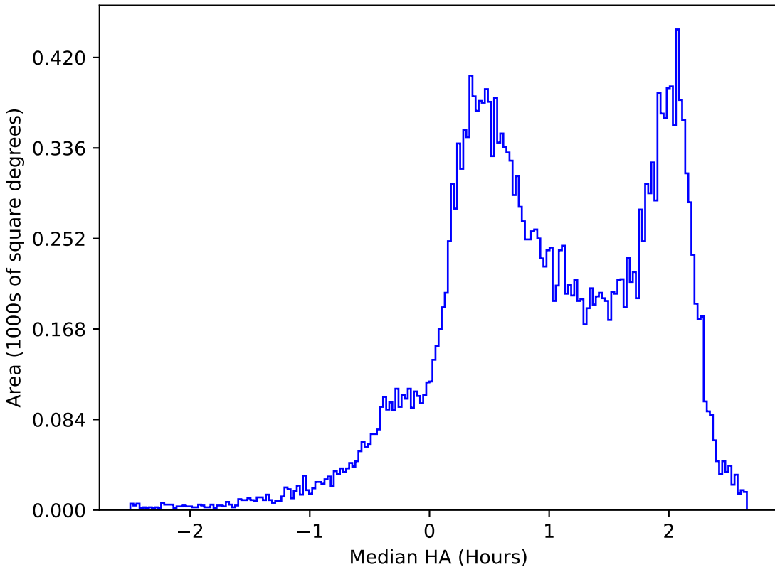
ddf_loaded_half_fl4_v3.4_10yrs All sky z band: Median HA
