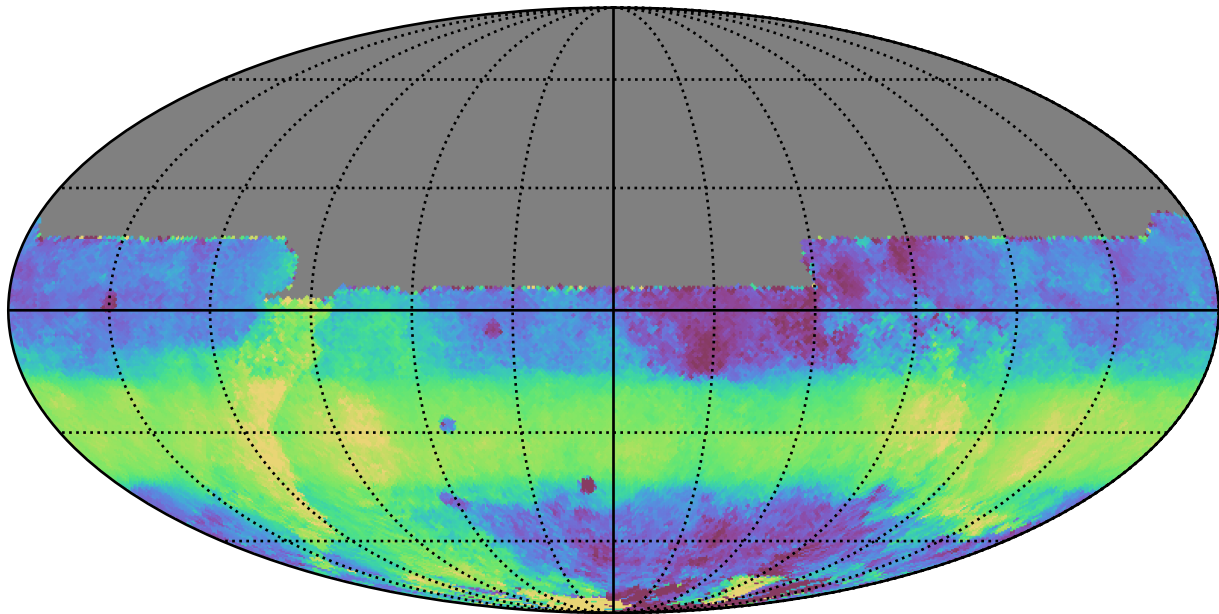
ddf_loaded_half_fl4_v3.4_10yrs All sky y band: Median HA
