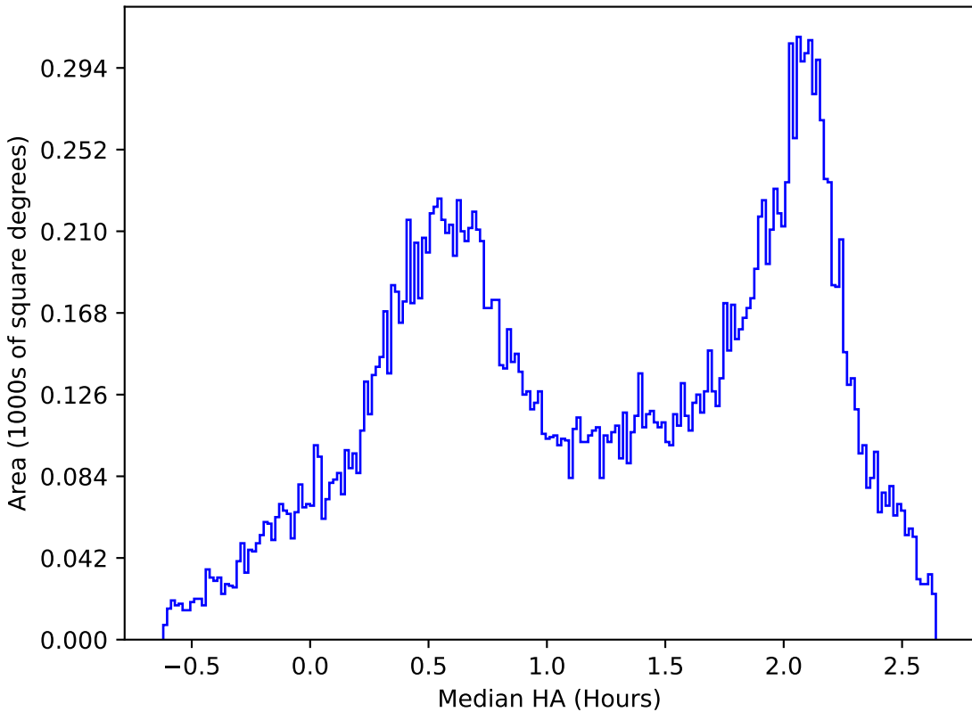
ddf_loaded_half_fl4_v3.4_10yrs All sky y band: Median HA
