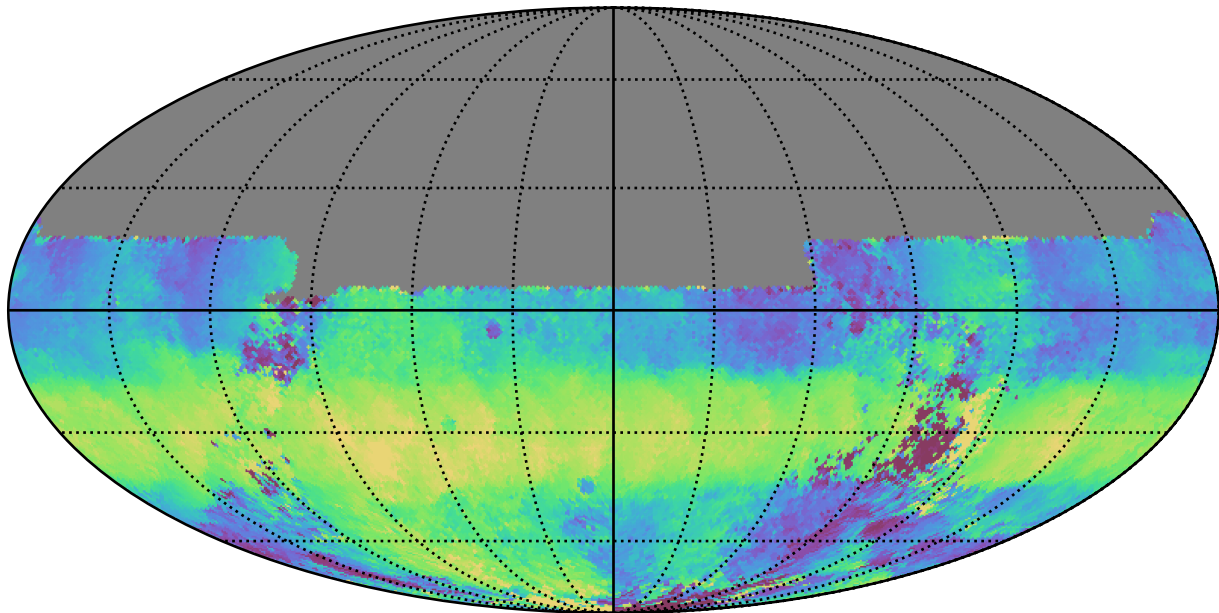
ddf_loaded_half_f14_v3.4_10yrs All sky u band: Median HA
