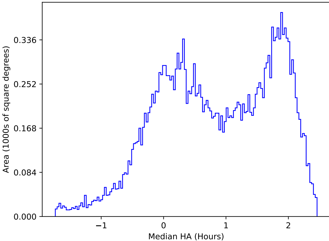
ddf_loaded_half_fl4_v3.4_10yrs All sky u band: Median HA
