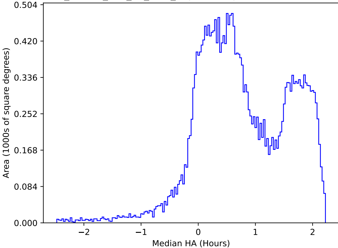
ddf_loaded_half_fl4_v3.4_10yrs All sky r band: Median HA
