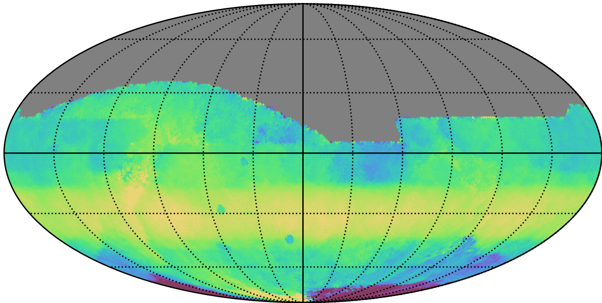
ddf_loaded_half_fl4_v3.4_10yrs All sky i band: Median HA
