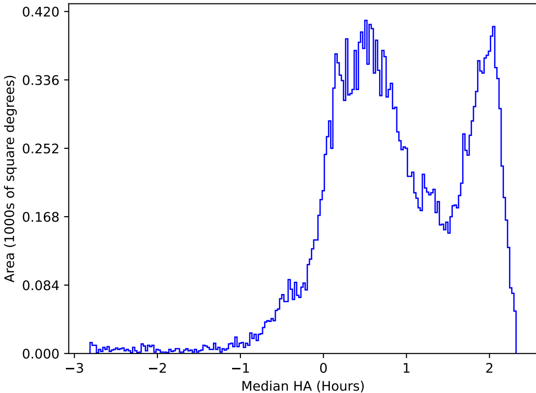
ddf_loaded_half_fl4_v3.4_10yrs All sky i band: Median HA
