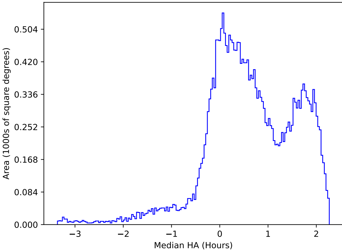
ddf_loaded_half_fl4_v3.4_10yrs All sky g band: Median HA
