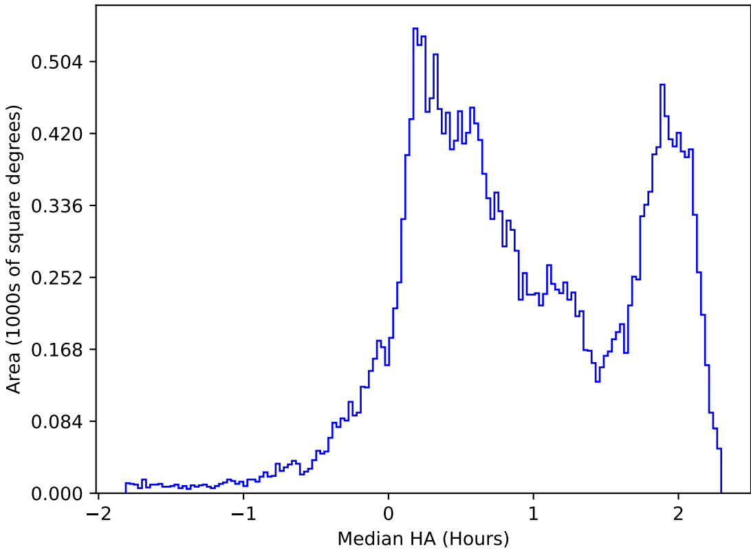
ddf_loaded_half_fl4_v3.4_10yrs All sky all bands: Median HA
