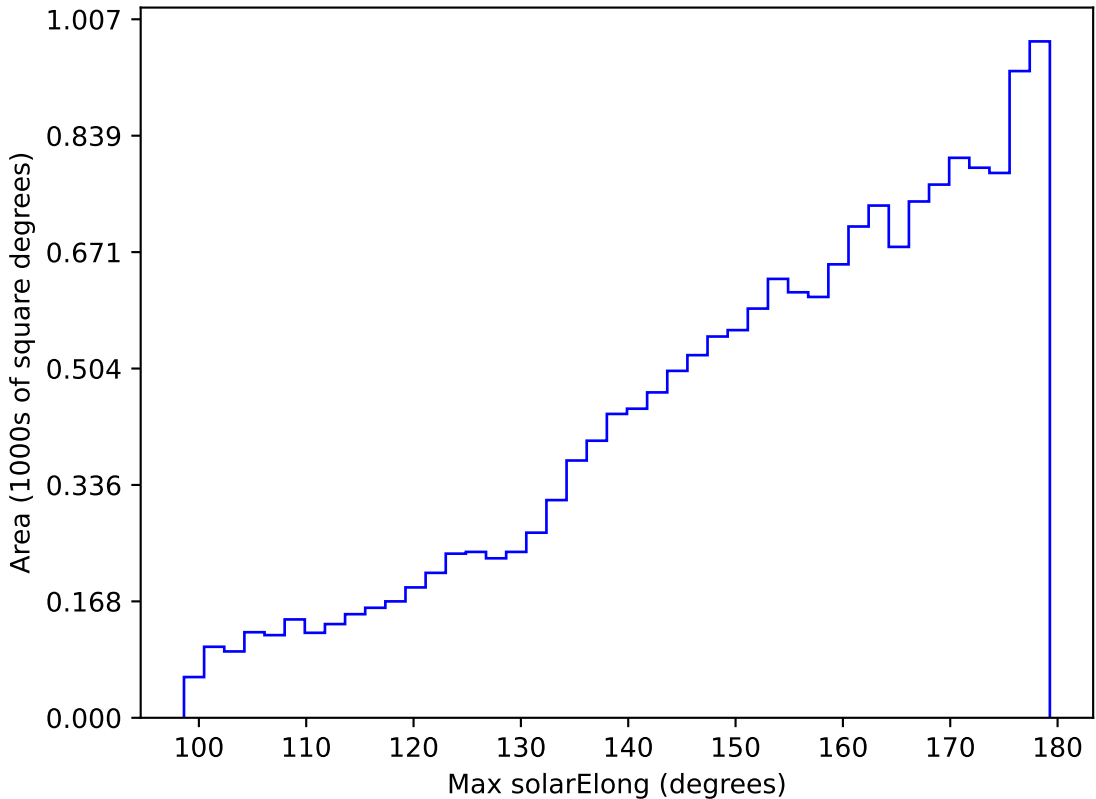
ddf_loaded_half_fl4_v3.4_10yrs WFD y band: Max solarElong
