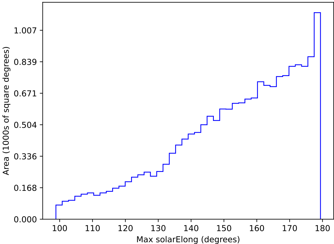
ddf_loaded_half_fl4_v3.4_10yrs WFD r band: Max solarElong
