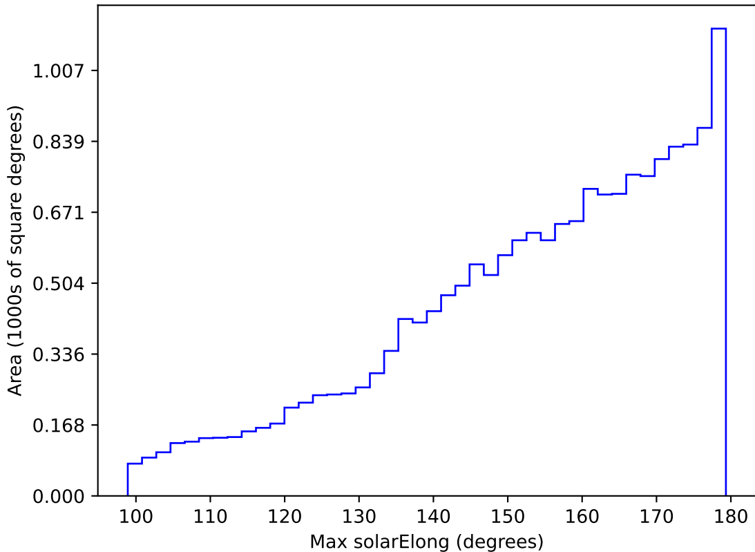
ddf_loaded_half_fl4_v3.4_10yrs WFD i band: Max solarElong
