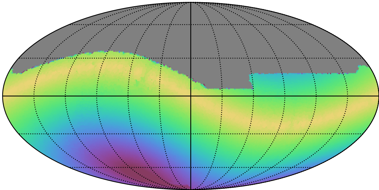
ddf_loaded_half_fl4_v3.4_10yrs All sky z band: Max solarElong
