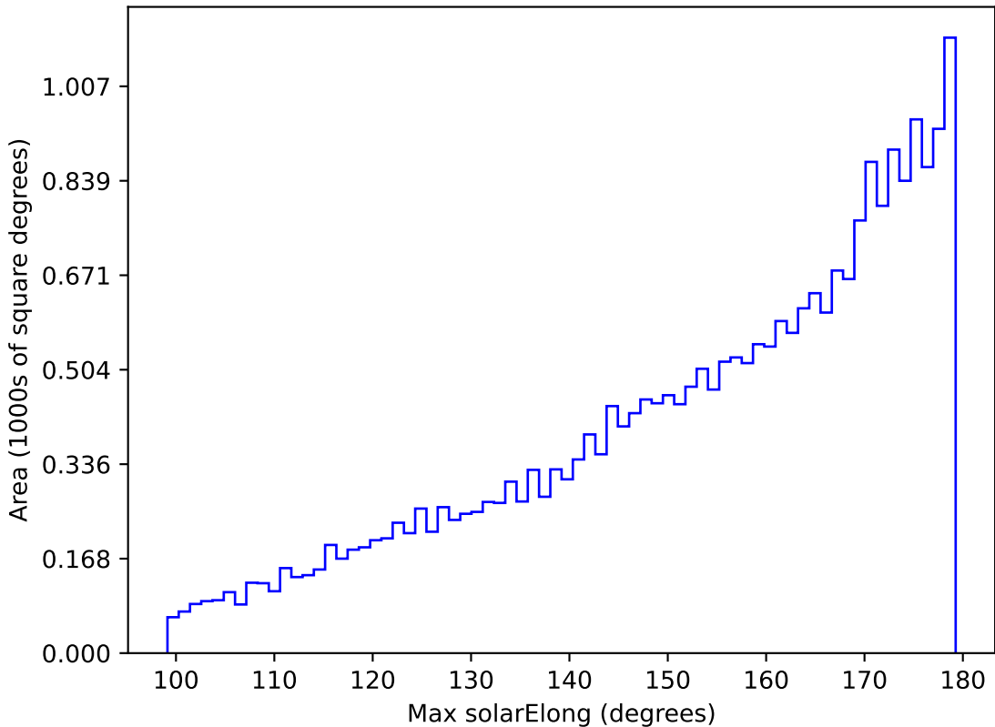
ddf_loaded_half_fl4_v3.4_10yrs All sky z band: Max solarElong
