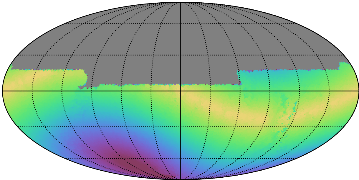
ddf_loaded_half_fl4_v3.4_10yrs All sky u band: Max solarElong
