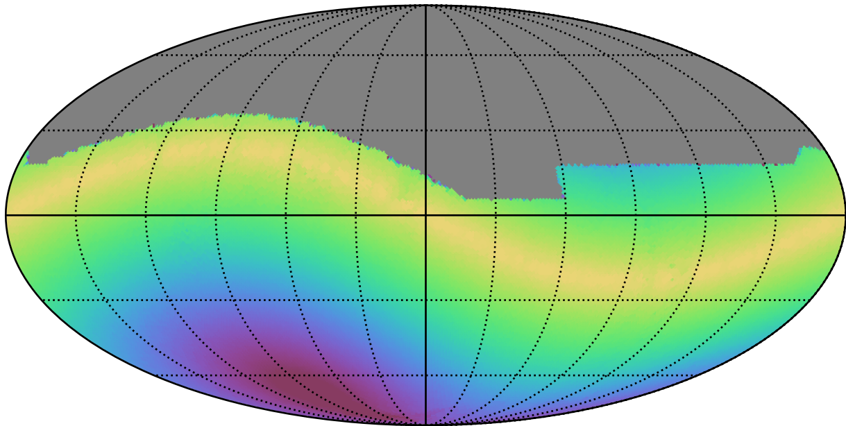
ddf_loaded_half_fl4_v3.4_10yrs All sky r band: Max solarElong
