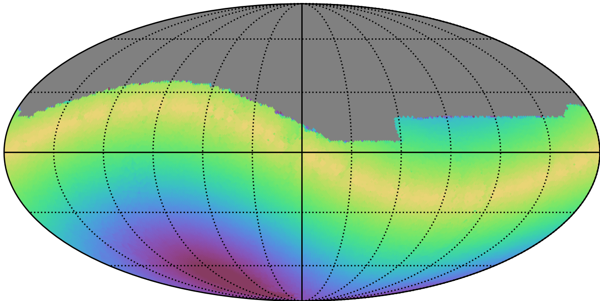
ddf_loaded_half_fl4_v3.4_10yrs All sky g band: Max solarElong
